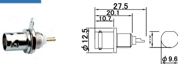
CN-22(E) BNC-BR
